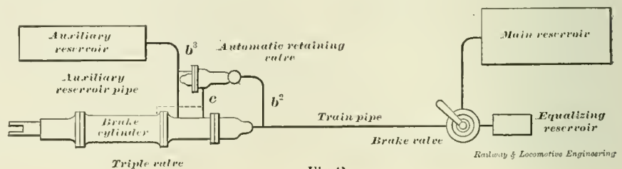
Fig. 2 AUTOMATIC RETAINING VALVE ATTACHED TO AIR-BRAKE SYSTEM.
